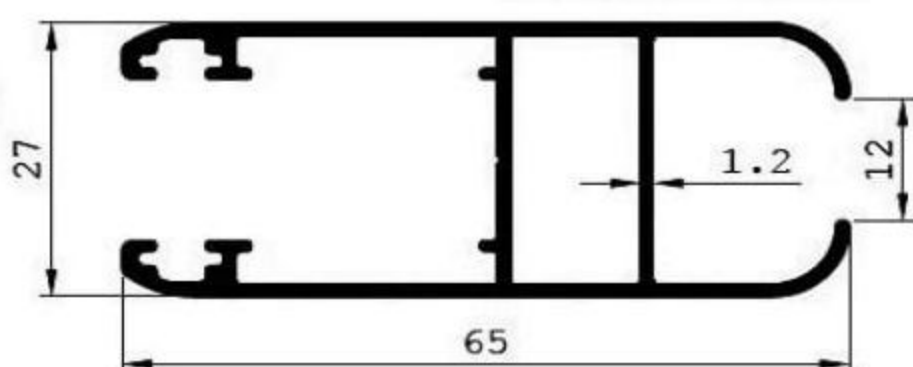
SINGLE GLASS SHUTTER
