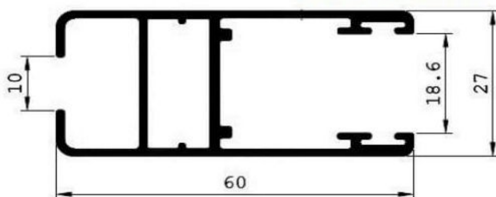
SINGLE GLASS SHUTTER
