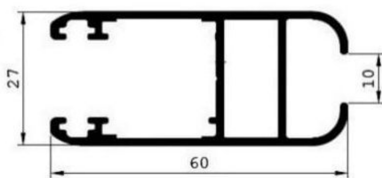
SINGLE GLASS SHUTTER
