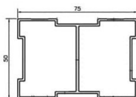
75 x 50mm SPECIAL PIPES Weight per 12Ft = 3.8 Kg.
