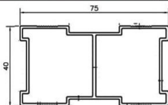
75 x 40mm SPECIAL PIPES Weight per 12Ft = 3.4 Kg.
