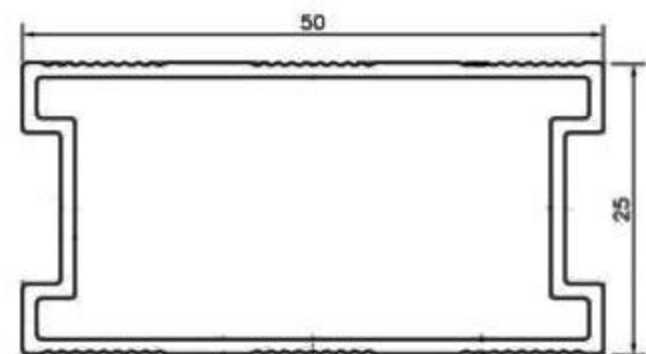
50 x 25mm SPECIAL PIPES Weight per 12Ft = 1.9 Kg.
