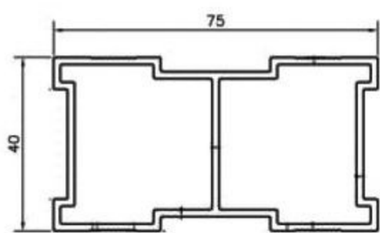
75 x 40mm SPECIAL PIPES Weight per 12Ft = 4.4 Kg.
