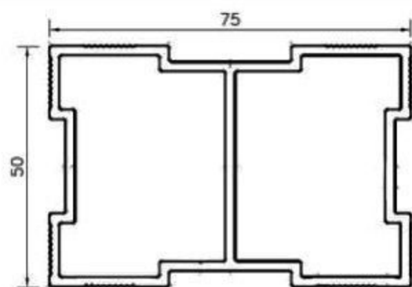
75 x 50mm SPECIAL PIPES Weight per 12Ft = 6 Kg.
