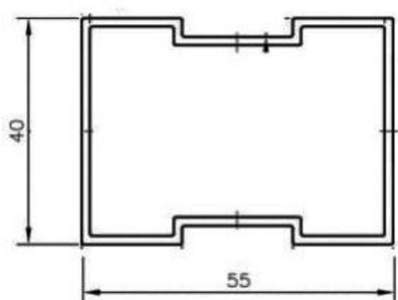
55x40mm SPECIAL PIPES Weight per 12Ft = 3.5 Kg.
