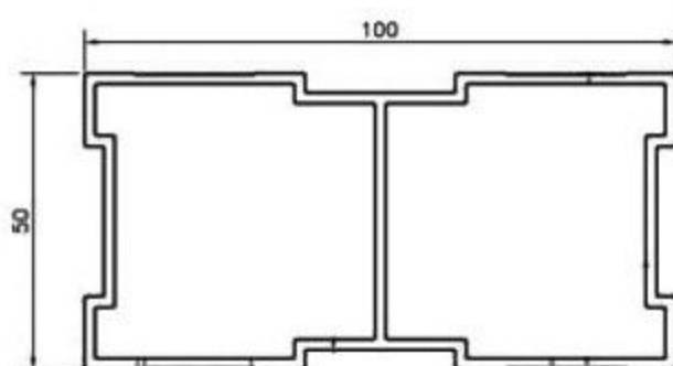
100 x 50mm SPECIAL PIPES Weight per 12Ft = 6.3 Kg.
