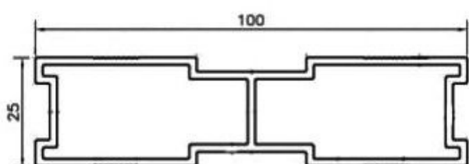
100 x 25mm SPECIAL PIPES Weight per 12Ft = 4.7 Kg.
