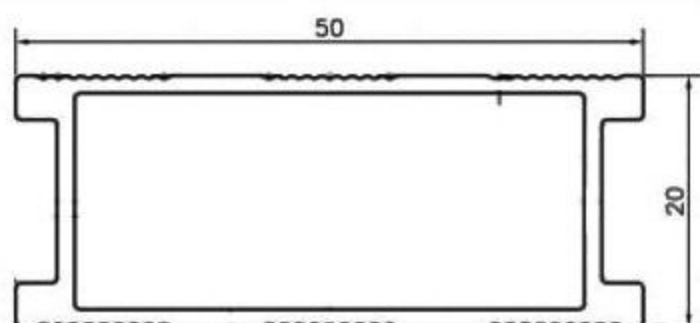
50 x 20mm SPECIAL PIPES Weight per 12Ft = 2.1 Kg.
