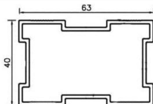
63 x 40mm SPECIAL PIPES Weight per 12Ft = 3.6 Kg.
