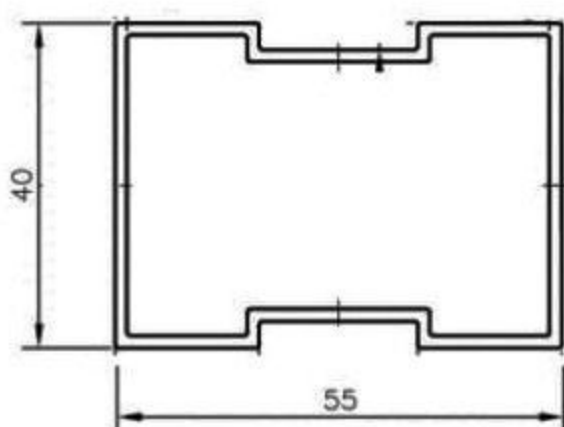
55x40mm SPECIAL PIPES Weight per 12Ft = 2.9 Kg.
