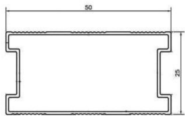
50 x 25mm SPECIAL PIPES Weight per 12Ft = 1.2 Kg.
