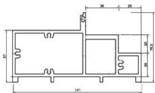
141 x 76.5mm SPECIAL PIPES Weight per 12Ft = 16.7 Kg.
